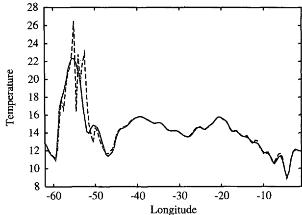
FIG. 6. Cross section at -39^\circ\text{N} of the surface temperature at 100 days showing the difference between the results of the two codes. The solid line is for the modified model and the dashed is for the standard model.
