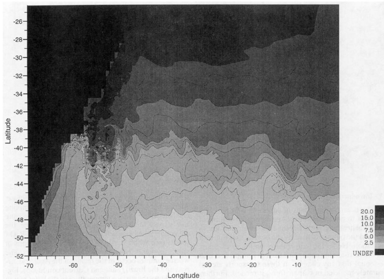
FIG. 1. An example of the output of FRAM for the surface temperature after 7 years of integration. There is significant under- and overshoot of the temperature near the South American coast.
